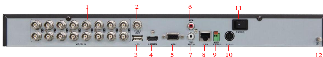
Figure 1.6 Rear Panel of SK-R916
