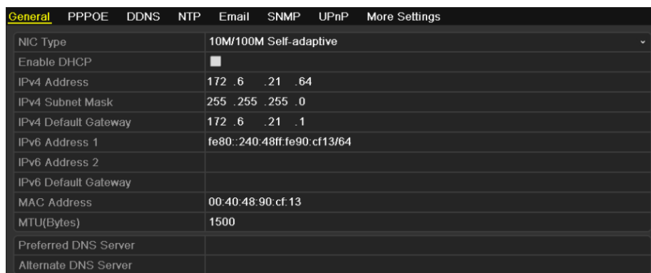
Figure 9.1 General Network Settings of SK-R904/SK-R908/SK-R916
